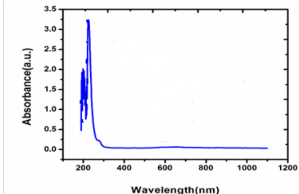
Fig. 4: Optical Analysis of CuS nanoparticles
