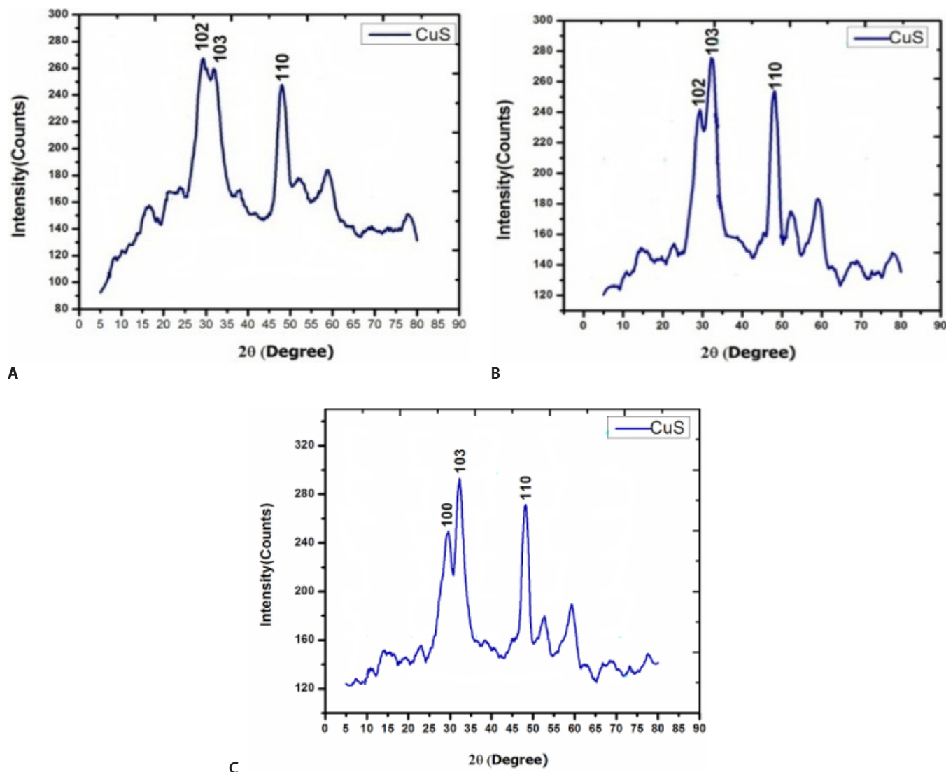
Fig. 1(A to C): XRD pattern for CuS nanoparticles; (A) At room temperature; (B) Calcination at 120°C; (C) Calcination at 200°C
