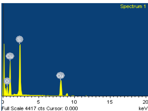
Fig. 3: EDAX Analysis of CuS nanoparticles
