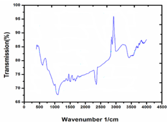
Fig. 5: FTIR spectrum of CuS nanoparticles
