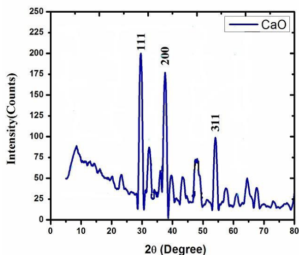
Fig. 1: XRD pattern of CaO nanoparticles
