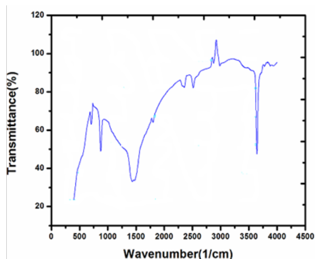
Fig.3: FTIR spectrum of CaO nanoparticles
