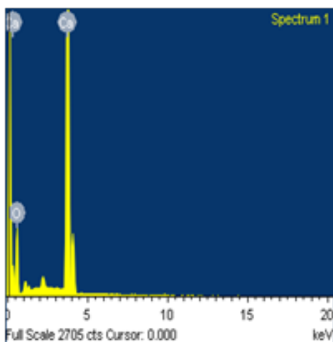
Fig. 2.2: EDAX Spectrum of CaO nanoparticles
