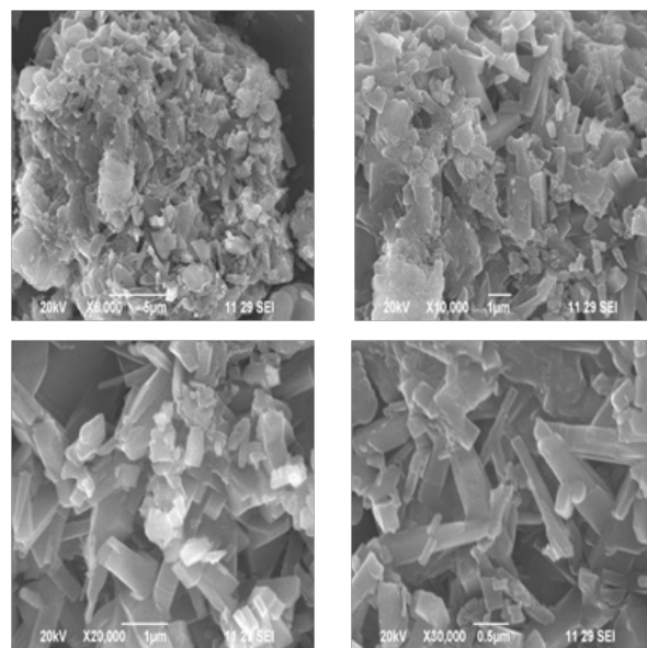
Fig. 3: SEM image of Rod like structure of MgO nanoparticles
