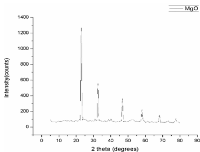
Fig. 1: XRD pattern of MgO nanoparticles
