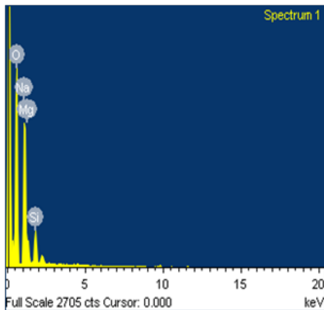
Fig. 4: Elemental composition of MgO nanoparticles
