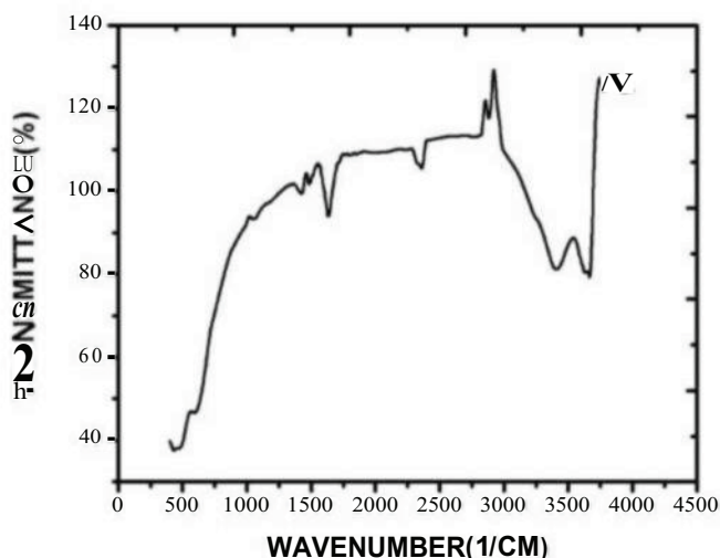
Fig. 2: FTIR image of Ni doped MgO nanoparticles
