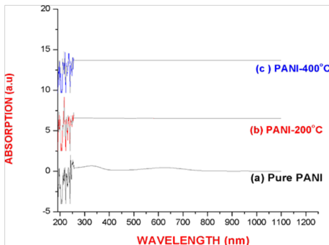
Fig 2: UV-Vis Spectra of (a) Pure PANI, (b) PANI (200°C) and PANI (400°C) Nanomaterial
