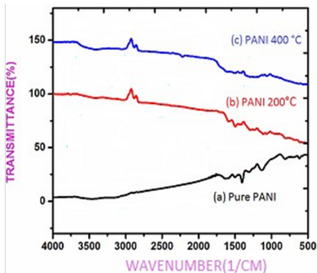
Fig. 1: FTIR Spectra of (a) Pure PANI, (b) PANI (200°C) and PANI (400°C)
