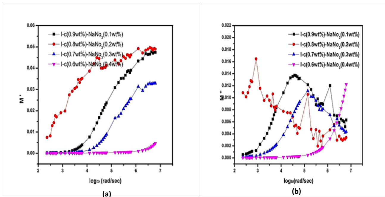
Figure 3 Variations of the (a) real part of electric modulus, M' and (b) imaginary part of electric modulus, M'' versus \log \omega for I – Carrageenan – sodium nitrate system
