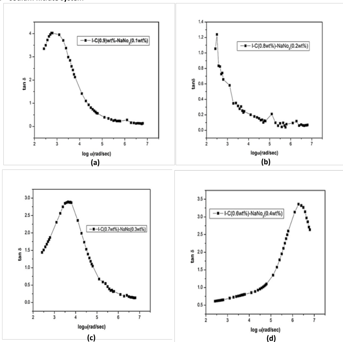
Figure 4 Variation of loss tangent spectra for prepared systems at room temperature
