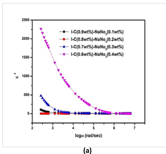
Figure 2 Variations of the (a) dielectric permittivity, \epsilon' and (b) dielectric loss, \epsilon'' versus \log \omega for I – Carrageenan – sodium nitrate system
